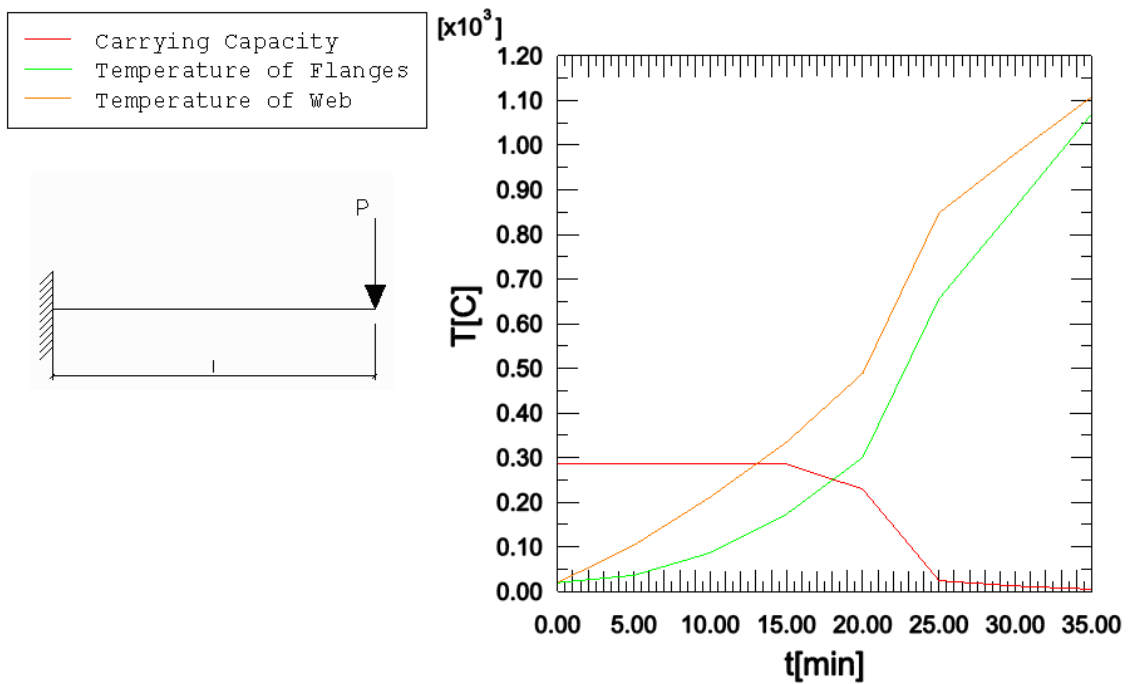
Fig. 16 Comparison of carrying capacity with temperature of web and flanges in 35min of fire
