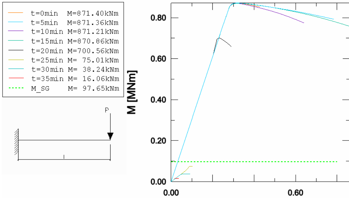
Fig. 15 Comparison of bending moments in encastre of beam for all types of analysis
