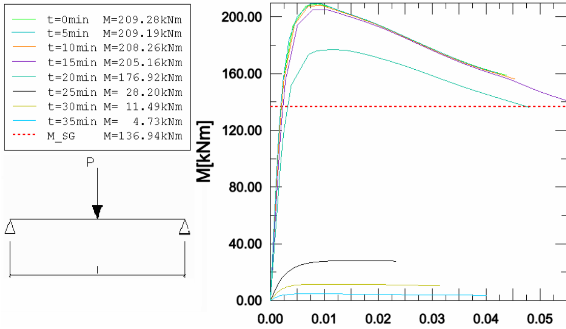
Fig. 11 Comparison of bending moments in middle section of beam for all types of analysis
