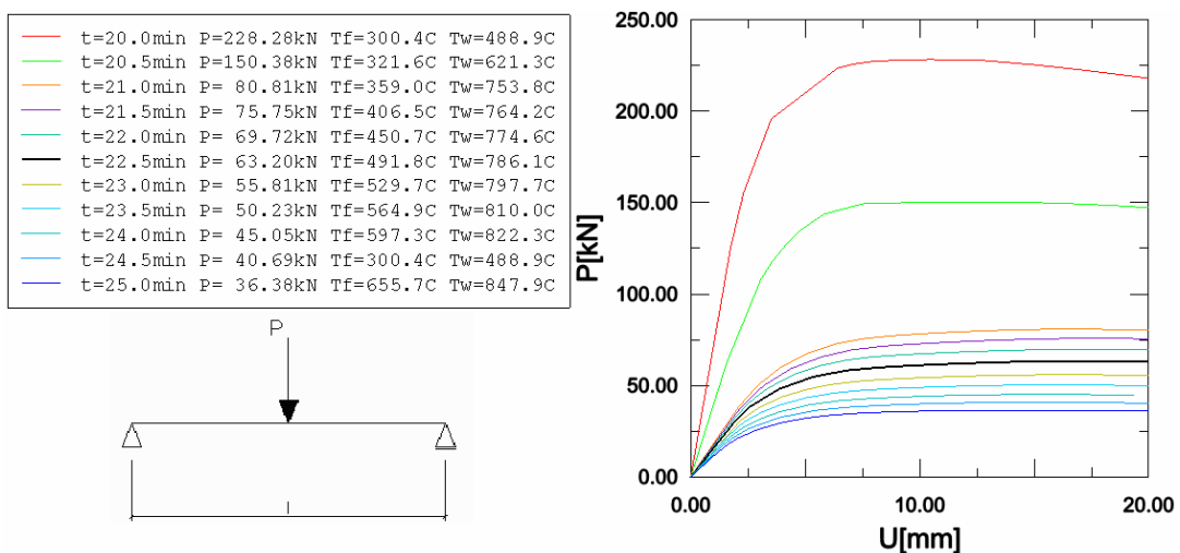
Fig. 10 Load – displacement curves for time from 20min to 25min of a fire
