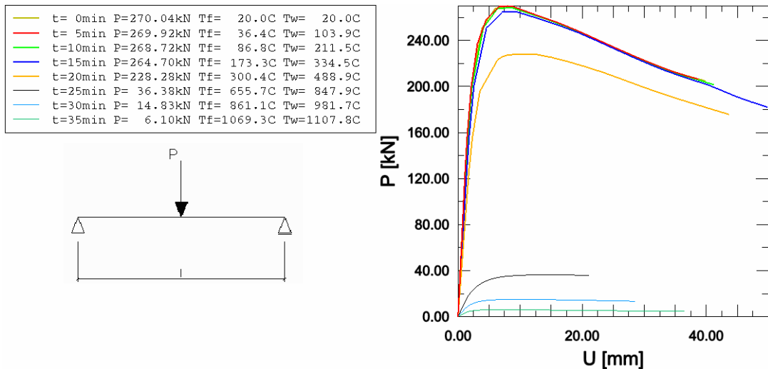
Fig. 9 Load – displacement curves for time from 0min to 35min of a fire
