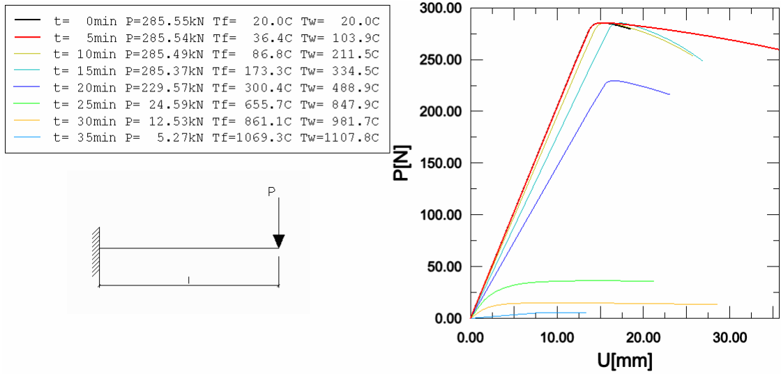
Fig. 13 Load – displacement curves for time from 0min to 35min of a fire
