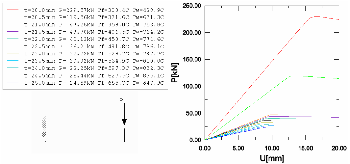
Fig. 14 Load – displacement curves for time from 20min to 25min of a fire
